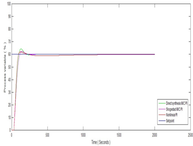
Fig. 4 Servo response of spherical tank at 60% operating point
