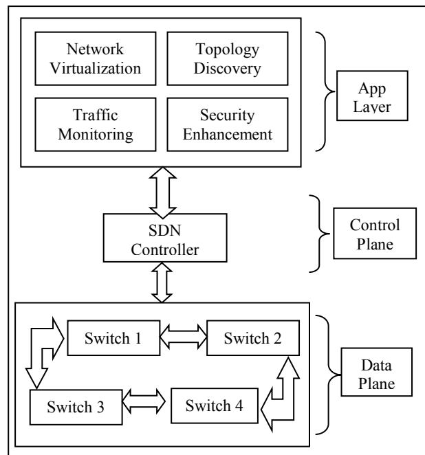
Fig. 1 SDN Architecture [9]
