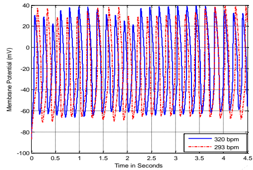
Fig.31. A.P of a Rabbit SAN coupled cell pair for GGJ at 0.1\mu S not in synchrony (Case 4)
