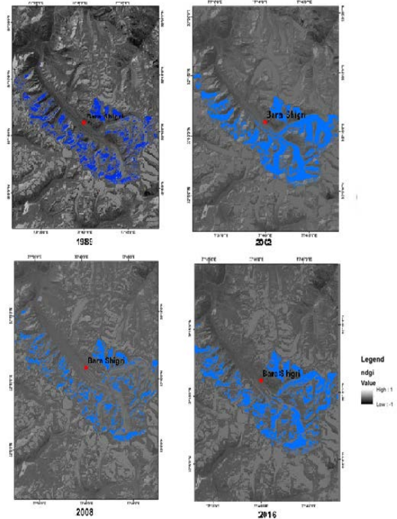
Fig. 8 Object-based analysis for detection of glacier melting and climate change on Bara Shigri glacier NDGI (Normalized Difference Glacier Index)
