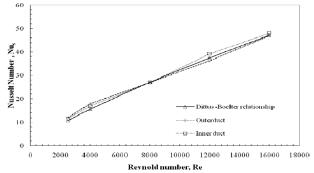
Fig. 7 Validation of inner and outer smooth duct of double duct solar air heater with Dittus-Boelter empirical correlation using RNG k-ε turbulence model.
