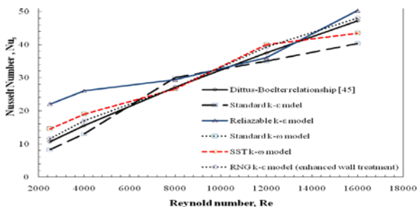
Fig. 6 Comparison between Nusselt number predicted using different CFD turbulence model with Dittus-Boelter empirical correlation for smooth duct of a solar air heater.
