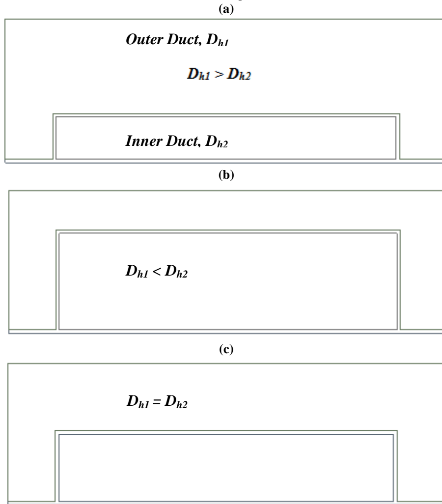
Fig. 2 Optimization of the double duct solar air heater (a) hydraulic diameter of the outer duct is greater than inner duct ( D_{h1} > D_{h2} ), (b) hydraulic diameter of the outer duct is less than inner duct ( D_{h1} < D_{h2} ) and (c) hydraulic diameter of the outer duct is equal to inner duct ( D_{h1} = D_{h2} ).
