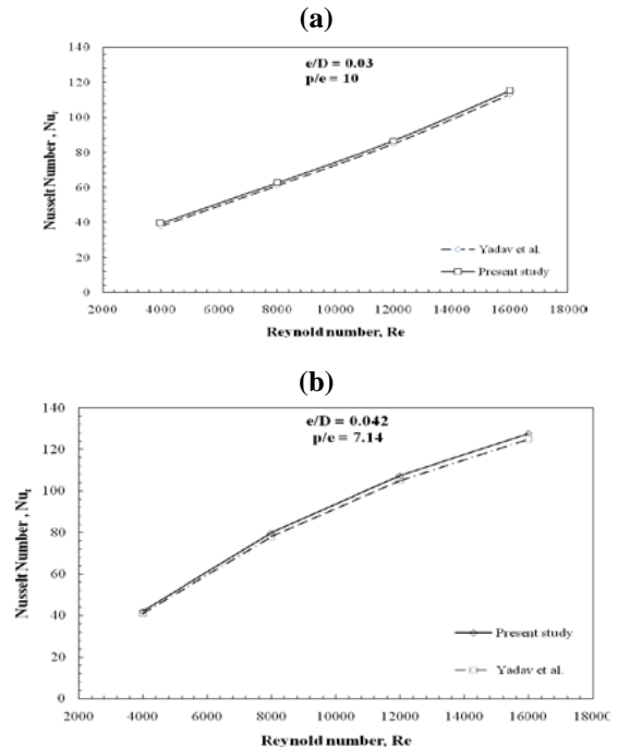
Fig. 8 Validation of CFD model with Yadav et al. for transverse rib roughness with (a) e/D =0.03, P/e = 10 and (b) e/D =0.042, P/e = 7.14
