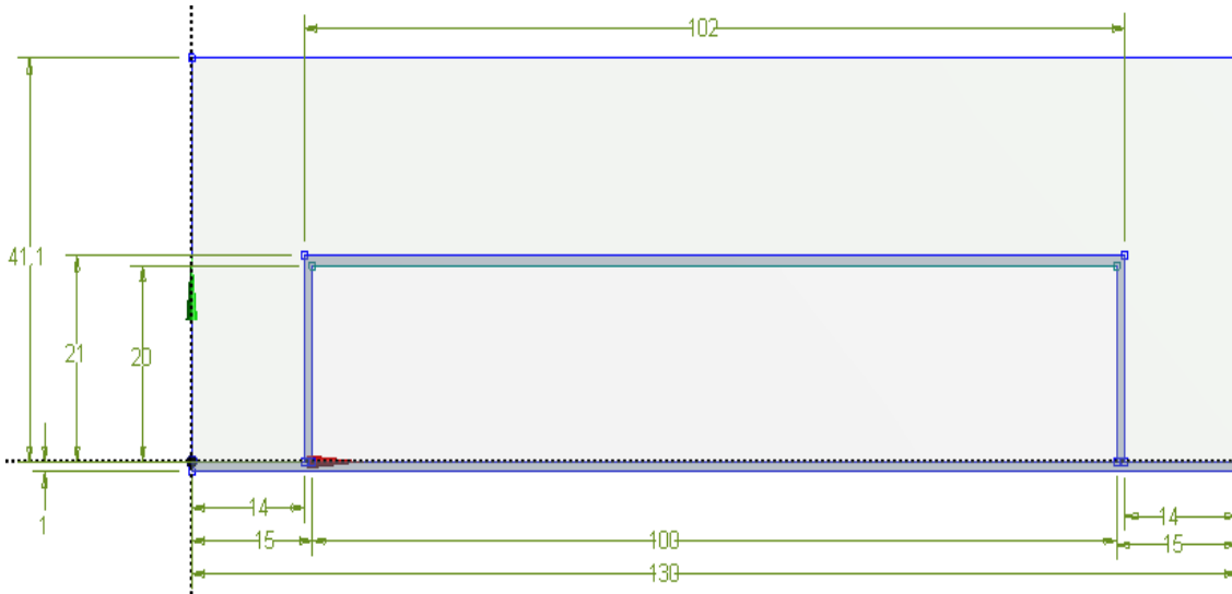
Fig. 5 Front view of proposed solar air heater with all dimensions in mm
