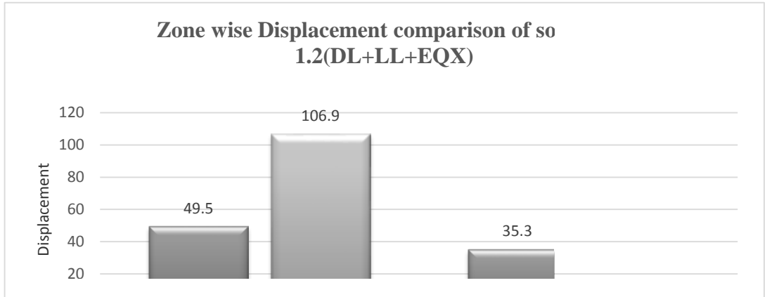
Fig.10 Showing zone wise displacement variation in soil-2
