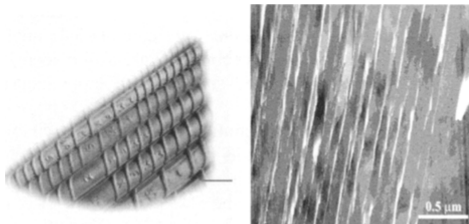
Fig.2 Nanostructure modified steel reinforcement TEM picture showing microstructure of Nano sheet of austenite in a carbide free lath of Martensite
