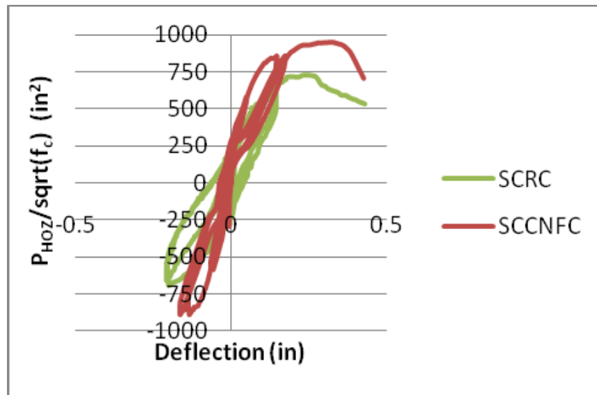
Fig. 1 Horizontal Force vs. Displacement Curves
