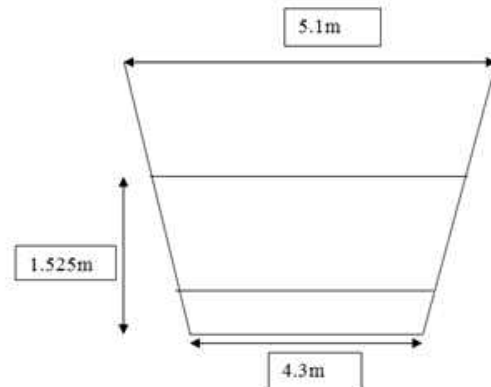
Fig. 3 Channel flowing half full
