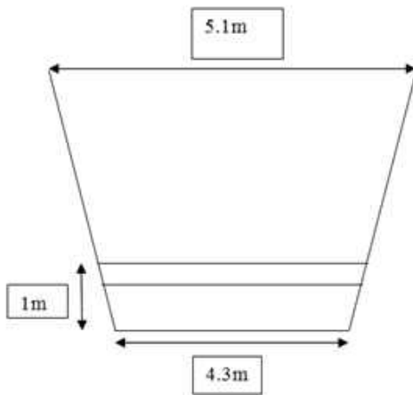
Fig. 4 Channel during lean period
