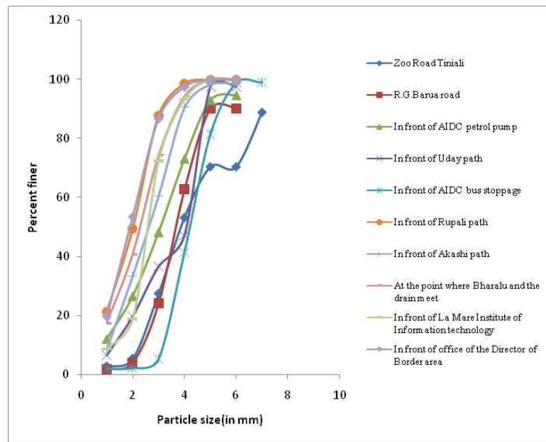
Fig. 1 Plot of particle size Vs percent finer of silt particles
