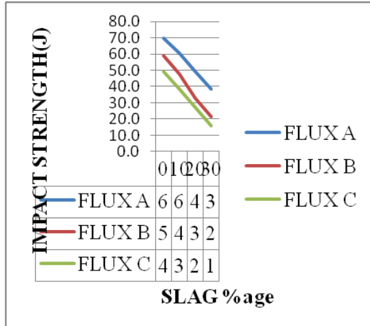
Fig. 6 Effect of slag %age on average impact strength of weld prepared by using flux A, B and C
